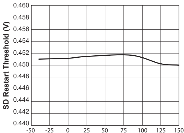
Ambient Temperature (°C) Figure 7.3 : SD Restart Threshold vs. Temperature
