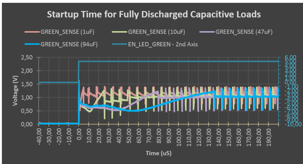
Figure 6. Startup Time for Fully Discharged Capacitive Loads (94 \mu F Input Capacitors)
