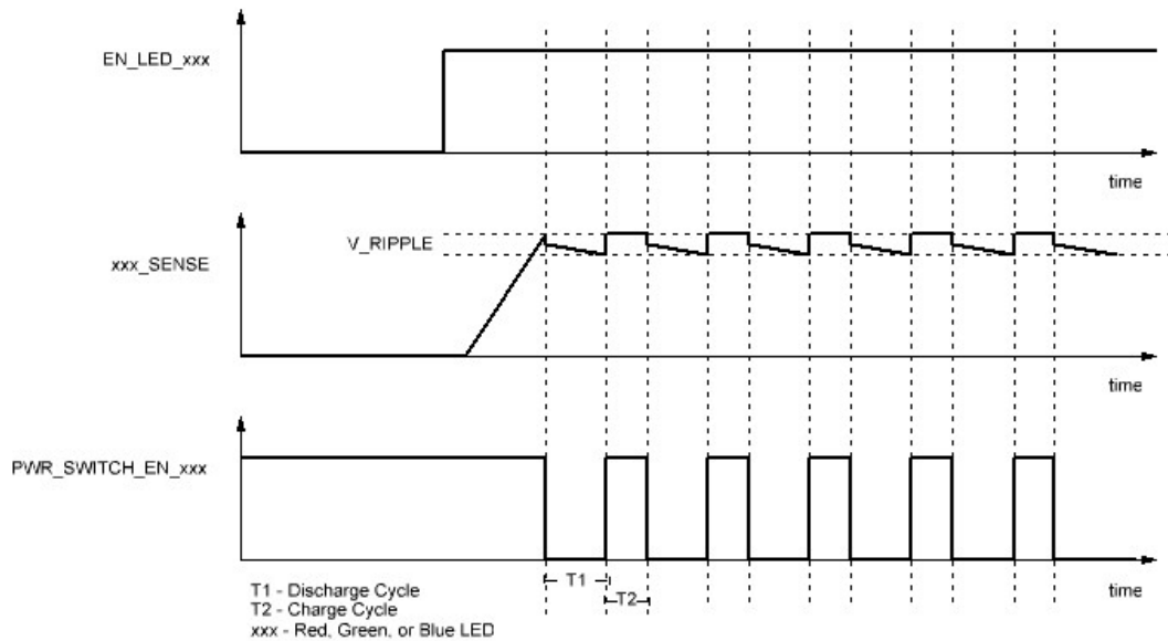
Figure 2. Constant Current Functional Waveform
