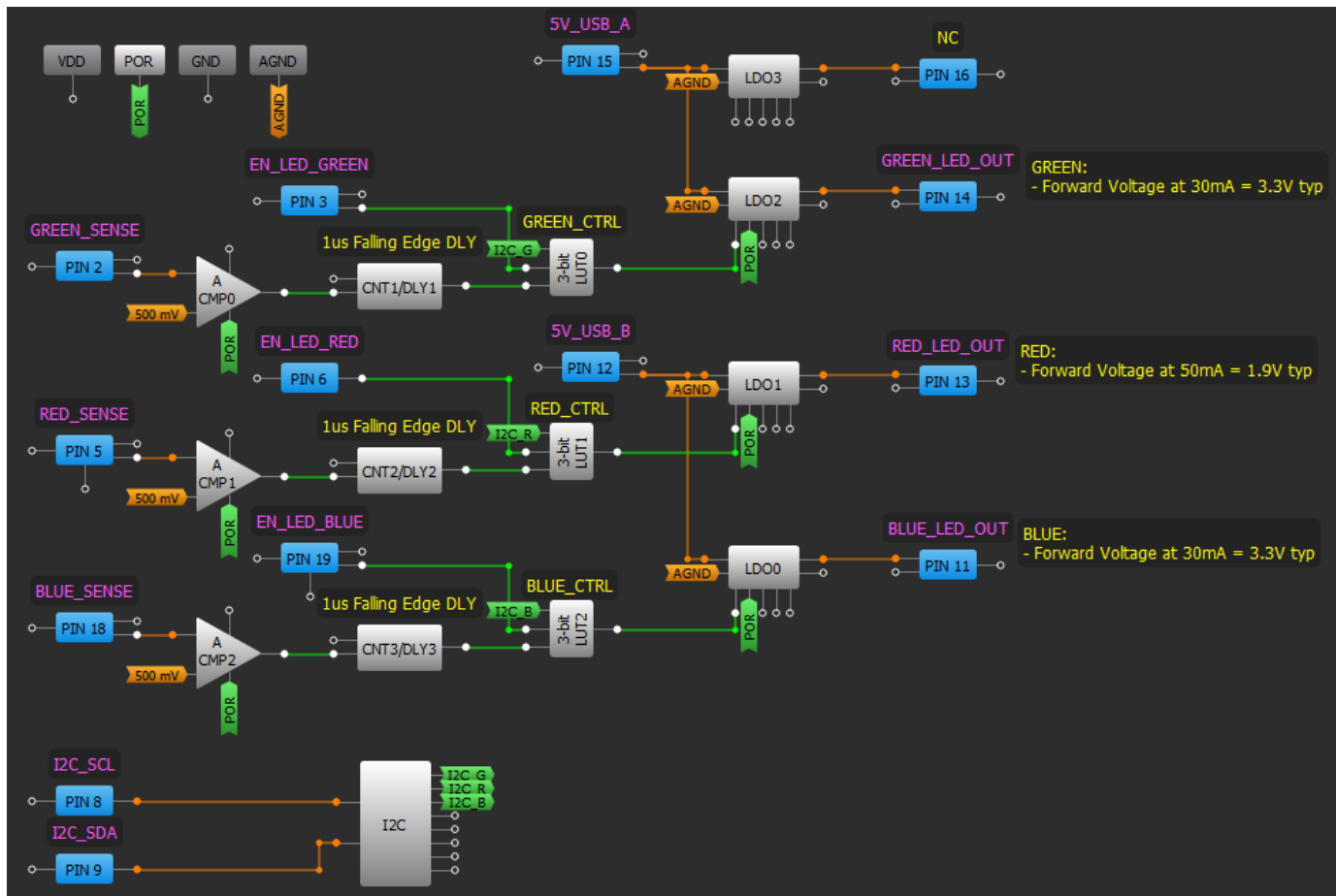
Figure 3. GreenPAK Constant Current RGB Driver Design
