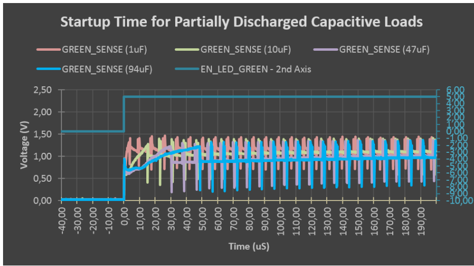
Figure 7. Startup Time for Partially Discharged Capacitive Loads (94 \mu F Input Capacitors)
