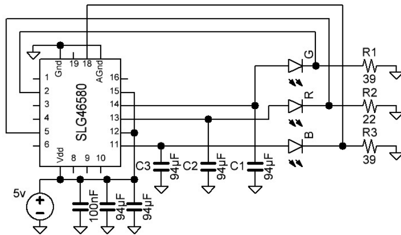
Figure 1. Constant Current RGB Driver Circuit Schematic
