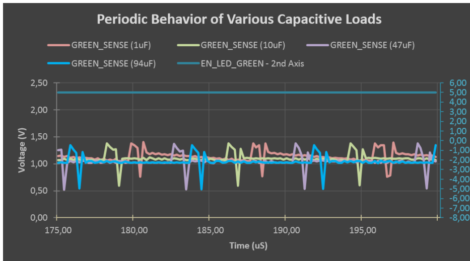
Figure 8. Periodic Behavior of the Various Capacitive Loads (94 \mu F Input Capacitors)
