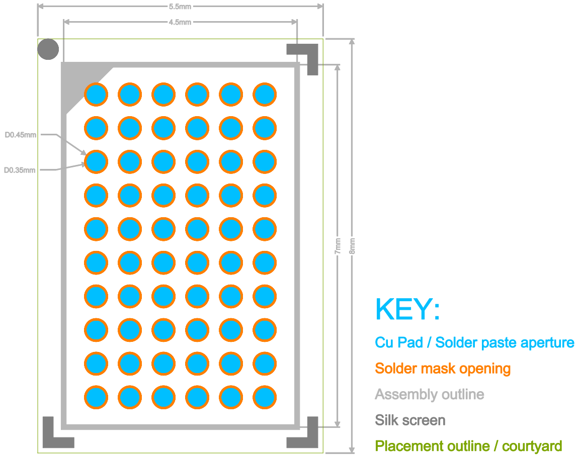
Figure 10: DA9141-A Footprint
