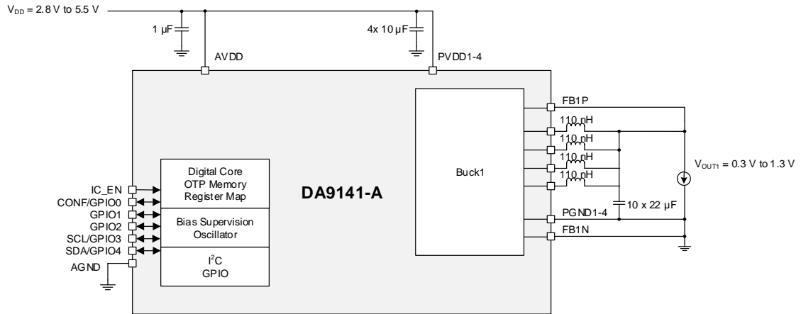
Figure 1: Block Diagram
